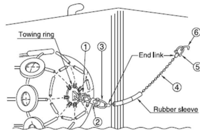
■ Table.6.B Installation Recommendation for Chain net type ( Type I) Medium and Large Size
